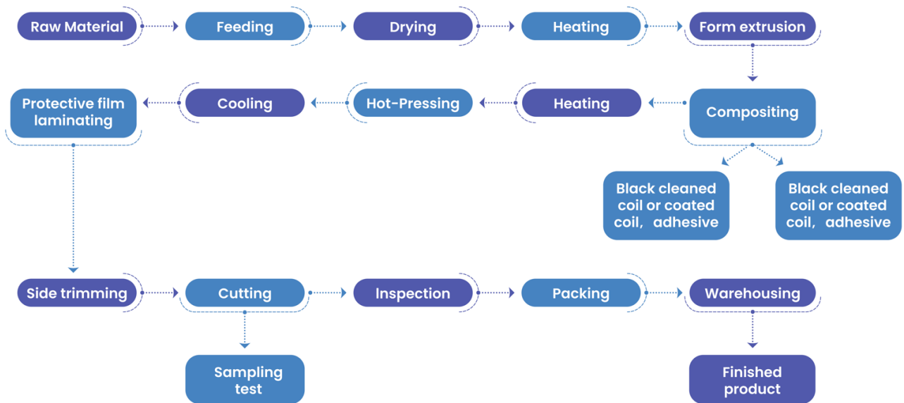
Figure 80. Manufacturing Process Analysis of Naked Eye 3D LED Display Screens
